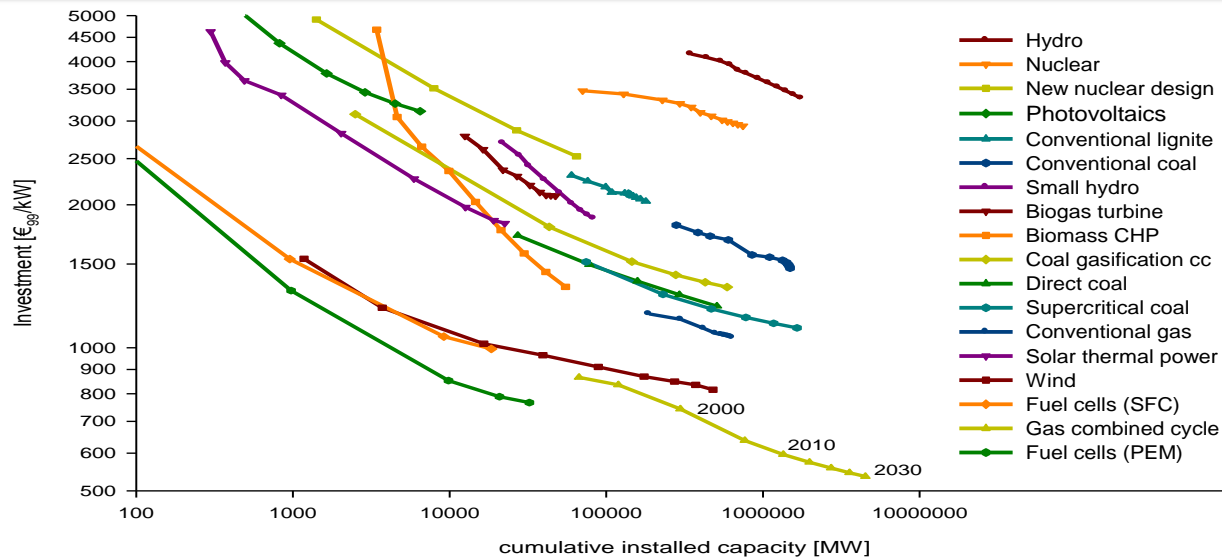
Learning curves for power generation technologies
